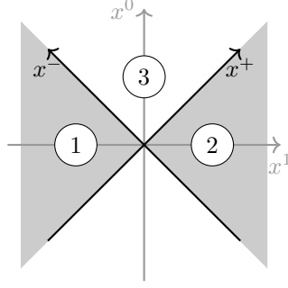
Figure 2.7: Partition of spacetime into light-cone quadrants. The quadrants where the Yang-Mills equations will be solved are identified as quadrants 1, 2 and 3. Adapted from [15].
