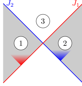
Figure 2.8: The same four quadrants with the support of current J_1 ( J_2 ) drawn as a red (blue) line. Future light-cones drawn from points where J_1 passes only occupy quadrants 1 and 3; future light-cones drawn from points where J_2 passes only occupy quadrants 2 and 3.
