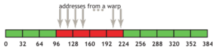
Figure 3: Coalesced access
