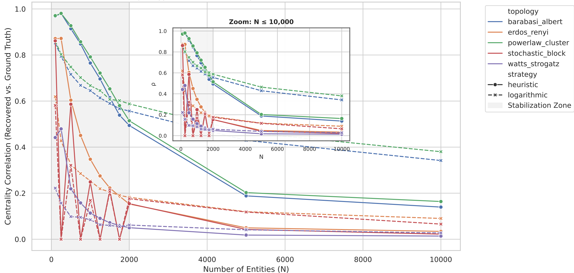
Topology Preservation Analysis (Pearson Correlation)
