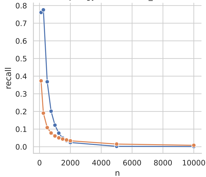
topology = stochastic_block
