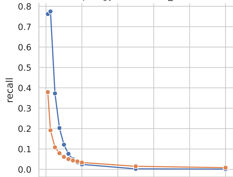
topology = barabasi_albert
