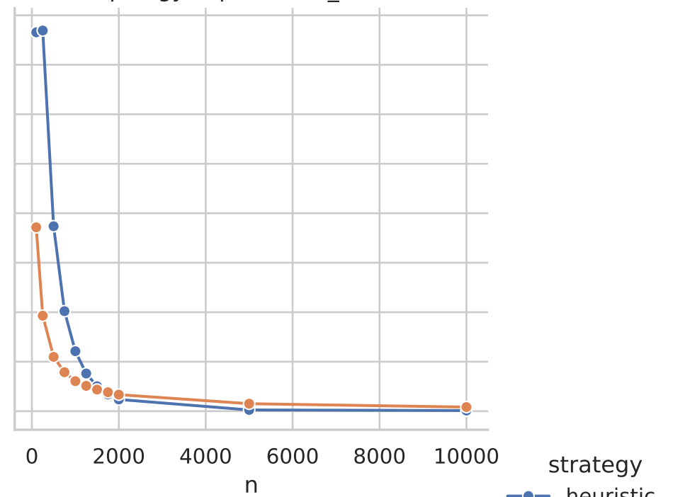
topology = powerlaw_cluster
