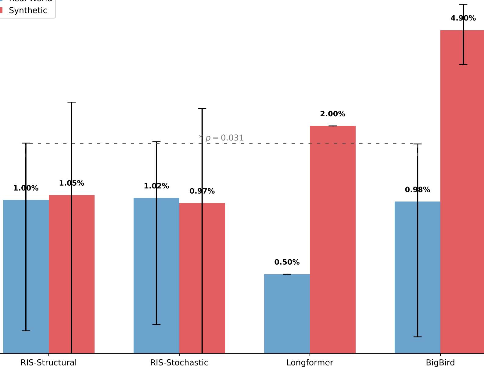
Topological Recovery: Average over 20000 Trials
