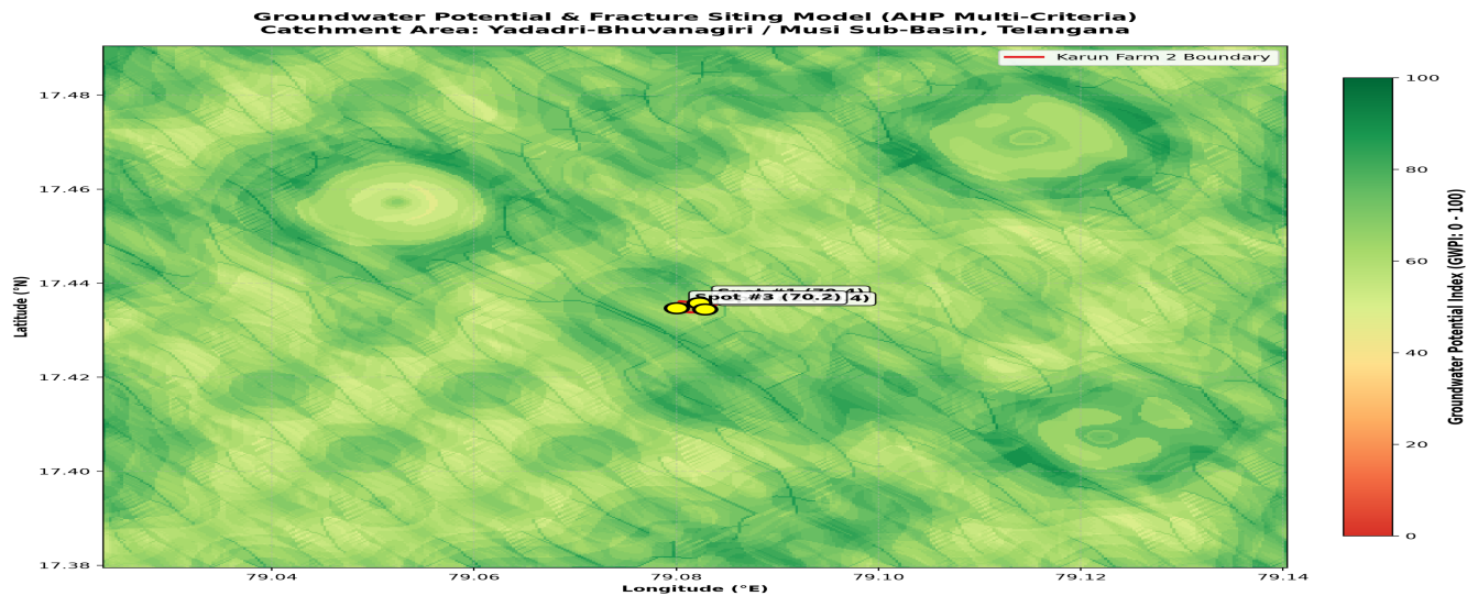
Figure 2: Regional 6km catchment hydrogeological model showing secondary NW-SE / NE-SW lineament corridors and Musi sub-basin drainage network.
