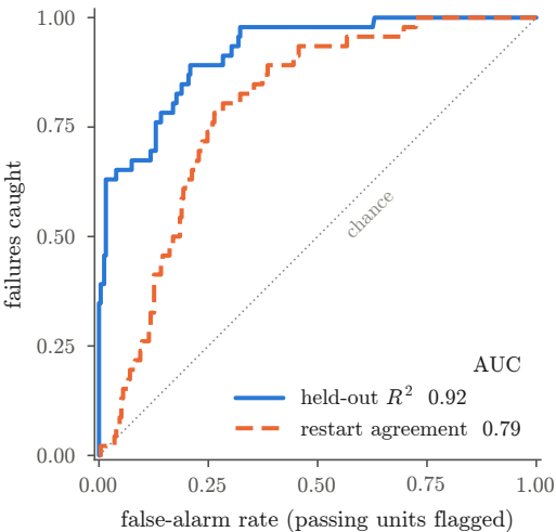
a GPT-2 small, layer 6: 300 units, 46 failures
