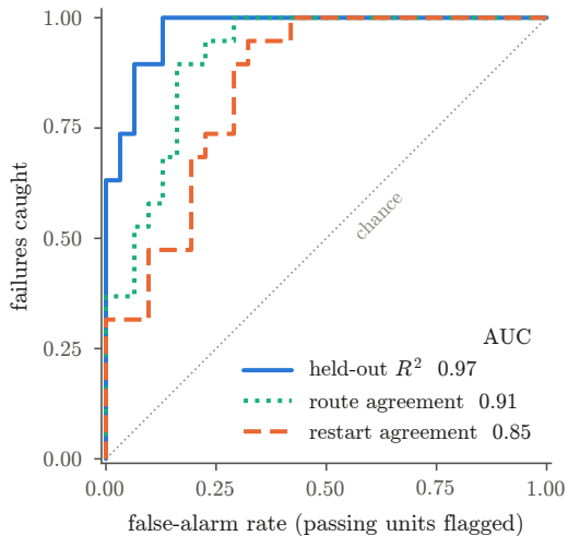
b Pythia-1.4B, layer 12: 50 units, 19 failures
