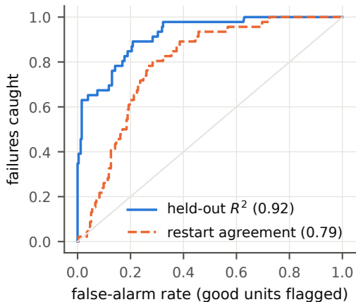
GPT-2 small L6, n=300, 46 failures
