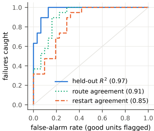
Pythia-1.4B L12, n=50, 19 failures
