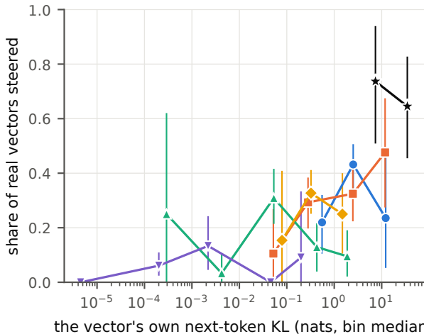
At the same KL, models steer at different rates
