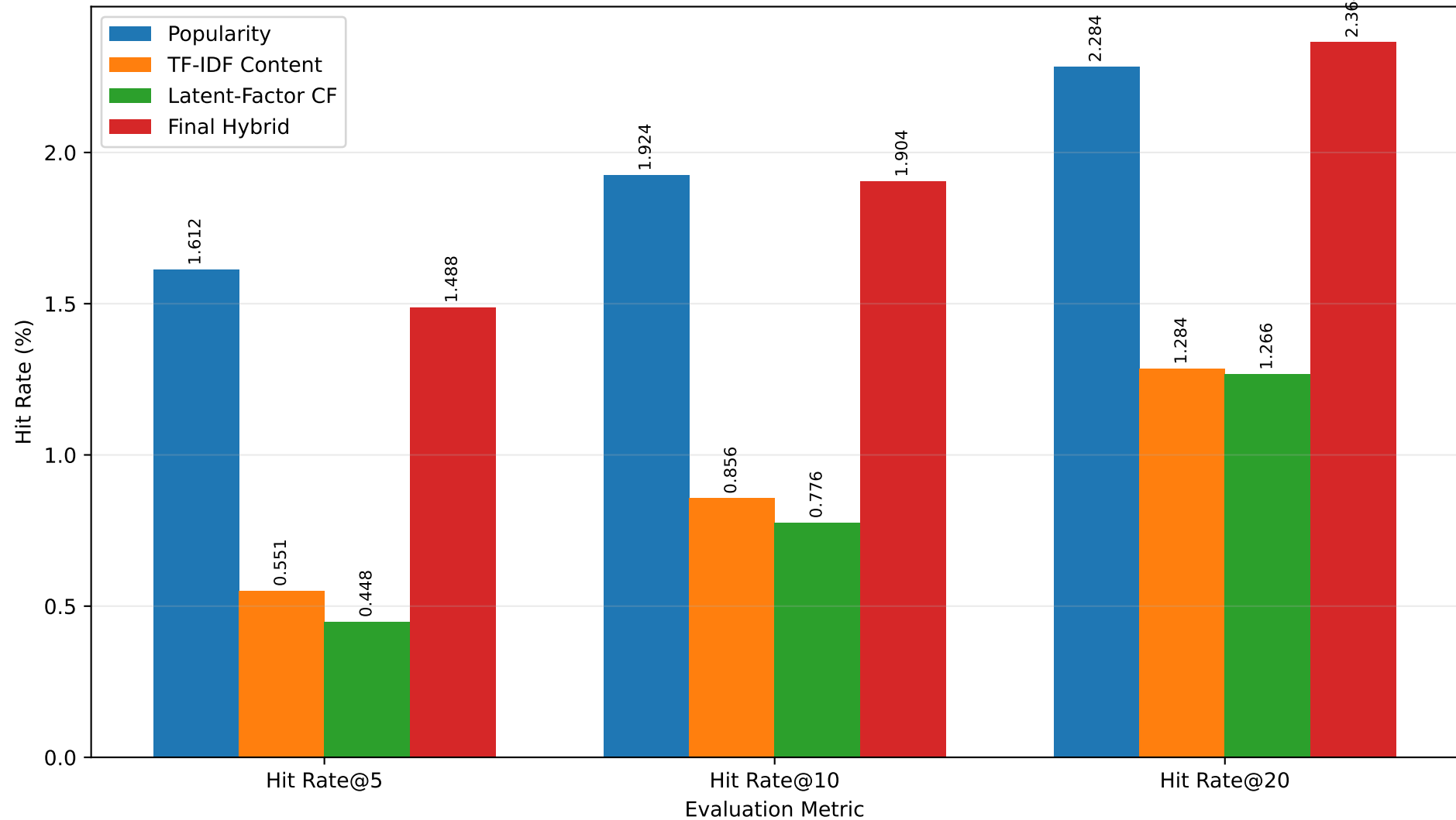
Positive Test-Set Hit Rate Comparison
