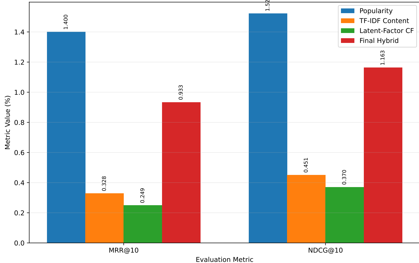
Positive Test-Set Ranking Quality Comparison
