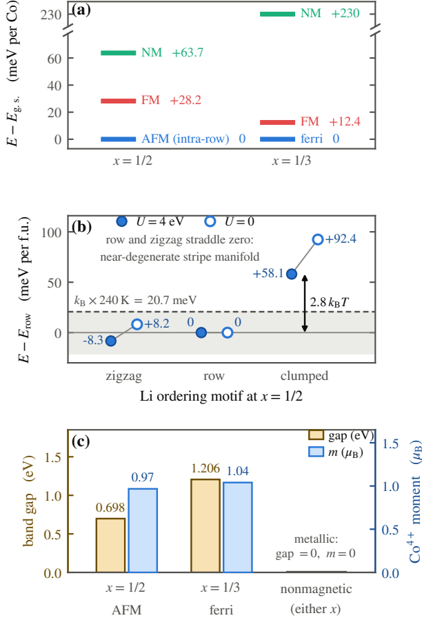
FIG. 4. Density-functional results for the ordered phases, at U = 4.0 eV on the cobalt 3d shell. (a) Energies of the magnetic configurations, per cobalt and relative to the ground state of each composition. At x = 1/2 the antiferromagnetic alignment within a \text{Co}^{4+} row is lowest, the ferromagnetic alignment lies 28.2 meV per cobalt above it, and the nonmagnetic solution lies 63.7 meV above; at x = 1/3 the ferrimagnetic arrangement is lowest, with the ferromagnetic one 12.4 meV and the nonmagnetic one 230 meV per cobalt above. (b) Energies of the three lithium motifs at x = 1/2 , per formula unit and relative to the row arrangement, filled markers at U = 4.0 eV and open markers at U = 0 . Clumping the stripes costs 58.1 meV per formula unit, above the reference line at k_B \times 240 K = 20.7 meV, while the zigzag variant changes sign between the two values of U and is therefore degenerate with the row arrangement. (c) Gap and \text{Co}^{4+} moment for each phase, 0.70 eV with 0.97 \mu_B at x = 1/2 and 1.21 eV with 1.04 \mu_B at x = 1/3 , against the nonmagnetic solutions, which have no gap at all; the panel prints the gaps to three decimals where the text rounds them to two. Moment, gap and charge order appear together, and removing the moment removes the other two.
