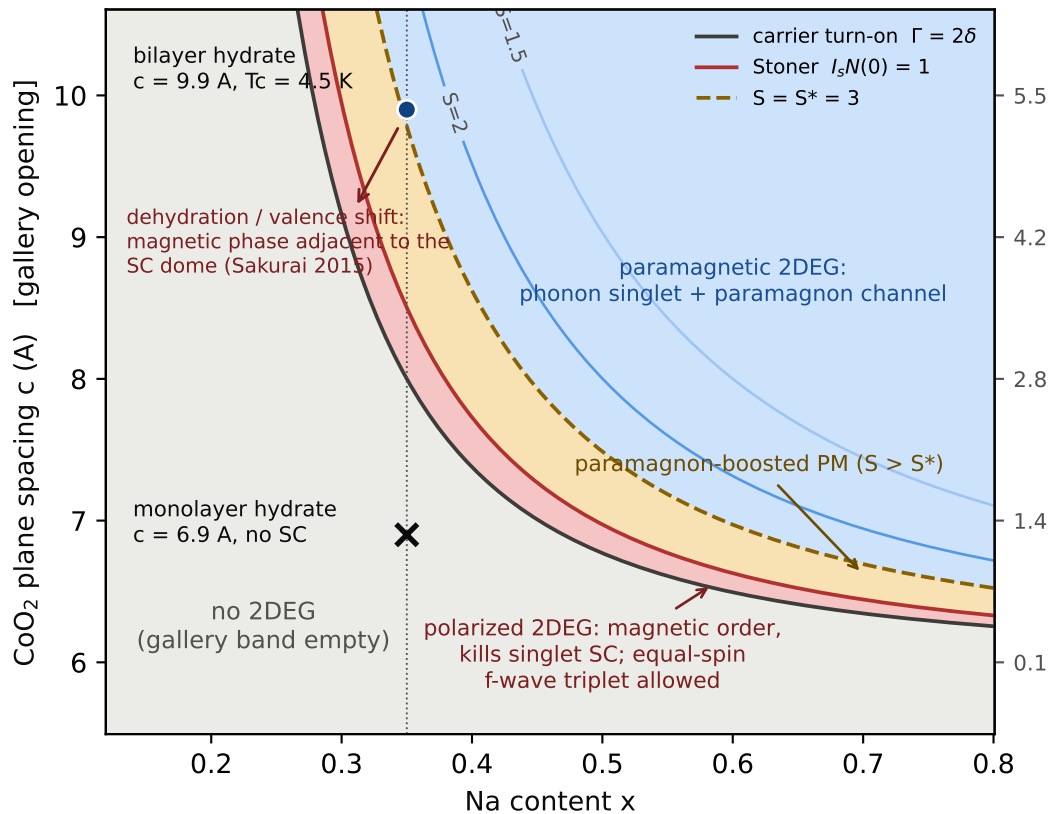
(a) Gallery-2DEG spin phase diagram (model, ansatz-labelled)
