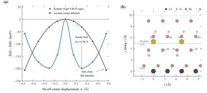
FIG. 8. The rigid-cage water demonstration. (a) Total energy E(\delta) of the off-centre sodium at c = 9.9 Å in the \sqrt{3}\times\sqrt{3} ( x = 1/3 ) cell, with a rigid four- \text{H}_2\text{O} solvation cage (hydrate) and with the water deleted (vacuum); points are QE total energies, curves guide the eye. Without water the curve runs away monotonically—the sodium chemisorbs onto a \text{CoO}_2 sheet, an unstable ( V''(0) < 0 ) mode with no bound state. With the rigid cage it becomes a bound double well (minima \approx \pm 0.30 Å, central barrier \approx 0.20 eV), a real confined mode of \hbar\omega_{\text{eff}} \approx 23 meV. The frozen cage re-binds the sodium but leaves the well deep; softening it into the pairing window is the work of the water’s motion (text). (b) The hydrate cell, drawn from the actual input coordinates (Appendix A), viewed along c : \text{CoO}_2 sheets at top and bottom, the sodium on its plane at c/2 , and the two-layer water cage between.
