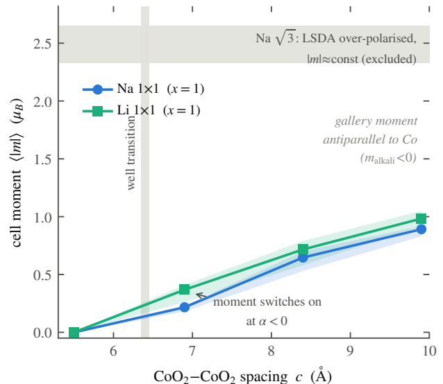
FIG. 9. The magnetic moment turning on with the well transition. Cell-integrated moment \langle |m| \rangle for \text{Na } 1 \times 1 and \text{Li } 1 \times 1 against gallery spacing; markers are the mean over the displacement scan and the bands its spread. The local moment switches on at the same spacing where \alpha turns negative, and the gallery moment is antiparallel to the cobalt. The \sqrt{3} cell is over-polarized in LSDA and is shown only as an excluded caveat band.
