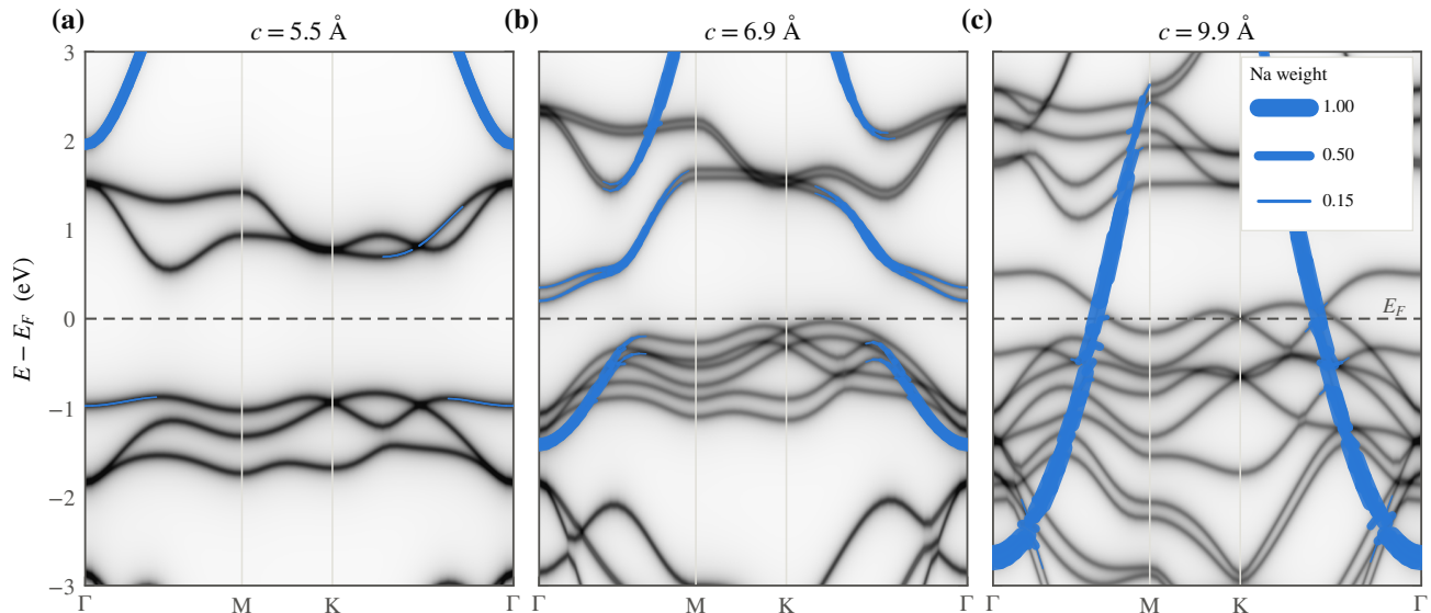
FIG. 4. The gallery band appears. Kohn-Sham spectral weight of Na 1 \times 1 along \Gamma -M-K- \Gamma at (a) 5.5, (b) 6.9 and (c) 9.9 Å, referenced to E_F (dashed). Grayscale is the total DFT spectral weight (all bands, both spins summed, each Lorentzian-broadened by \Gamma = 40 meV); the blue fatband is the sodium-orbital projected weight from PROJWFC, its width proportional to the sodium character (key in (c)). At 5.5 Å the x = 1 cell is a band insulator and the sodium band lies \approx 2 eV above E_F ; by 9.9 Å a band of \sim 90\% sodium character has descended through E_F —the interlayer 2DEG as a single band. Above the transition the cell is weakly spin-polarized ( 0.8 \mu_B at 9.9 Å), so this band is spin-split; both spins are summed here. No self-energy is applied: this is bare Kohn-Sham weight, not a renormalized quasiparticle spectrum.
