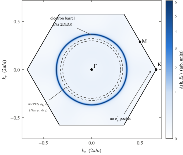
FIG. 5. Fermi surface at 9.9 Å. A(\mathbf{k}, E_F) in the k_z = 0 plane of the \text{Na } 1 \times 1 hexagonal BZ, from the dense 24 \times 24 \times 8 NSCF eigenvalues, symmetry-completed with the C_{6v} operations and Lorentzian-broadened at E_F (50 meV, both spins summed). The calculation gives a single electron barrel around \Gamma (the sodium 2DEG) and no e_g' pockets at K. ARPES on the anhydrous parent \text{Na}_{0.73}\text{CoO}_2 [4] sees the same topology—a single a_{1g} barrel around \Gamma (dashed, its measured k_F \approx 0.65\text{--}0.70 \text{ \AA}^{-1} ) and no e_g' pockets, the e_g' band sitting \approx 85 meV below E_F . Our barrel is sodium- rather than cobalt-derived and the composition differs, so we compare topology and size, not band identity; the barrels are of comparable radius. The measured a_{1g} velocities ( v_F \approx 0.3/0.6 \text{ eV \AA} along \Gamma\text{--K}/\Gamma\text{--M} ) are \sim 2\times below band theory, a renormalization our self-energy-free Kohn–Sham map does not carry.
