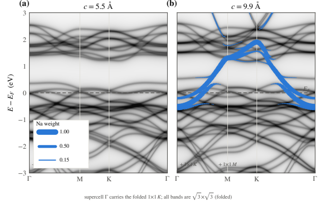
FIG. 6. The gallery band at the physical composition, x = 1/3 (supplementary). Kohn–Sham spectral weight of the \text{Na } \sqrt{3} \times \sqrt{3} cell at (a) 5.5 and (b) 9.9 Å, built exactly as in Fig. 4 (grayscale total weight, blue sodium fatband, both spins summed, 40 meV). The result mirrors the x = 1 case: no sodium weight at E_F at 5.5 Å, a strong sodium band through E_F at 9.9 Å. These are supercell bands and every one is a fold of the primitive zone; lacking the plane-wave coefficients for a weight-resolved unfolding, we do not draw an unfolded dispersion but mark the folding relations instead—the 1 \times 1 K point folds onto the supercell \Gamma and the 1 \times 1 M point onto the supercell M. Read every band here as folded.
