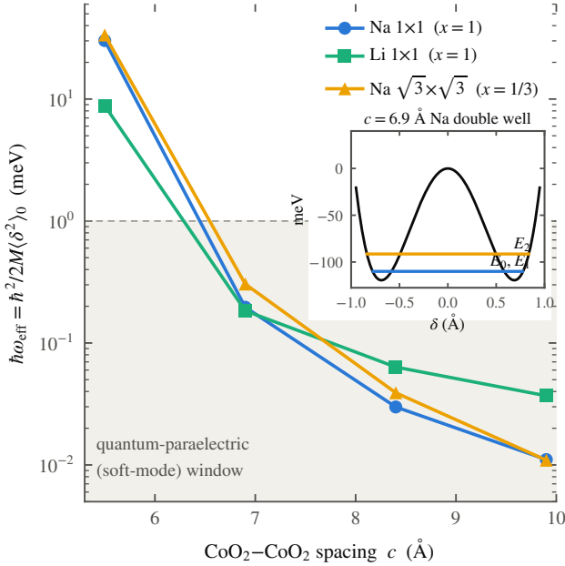
FIG. 7. The sodium mode softening. Effective zero-point frequency \hbar\omega_{\text{eff}} = \hbar^2/2M\langle\delta^2\rangle_0 of the quantized alkali mode, from an exact one-dimensional solution of the fitted wells at the physical masses. It collapses by three orders of magnitude across the transition, from a stiff \sim 30 meV single-well mode into a sub-meV soft mode as the gallery opens, entering a quantum-paraelectric window. Inset: the lowest levels in the 6.9 Å sodium double well, with the near-degenerate tunnelling doublet E_0, E_1 and the even overtone E_2 that carries the quadratic electron-phonon coupling.
