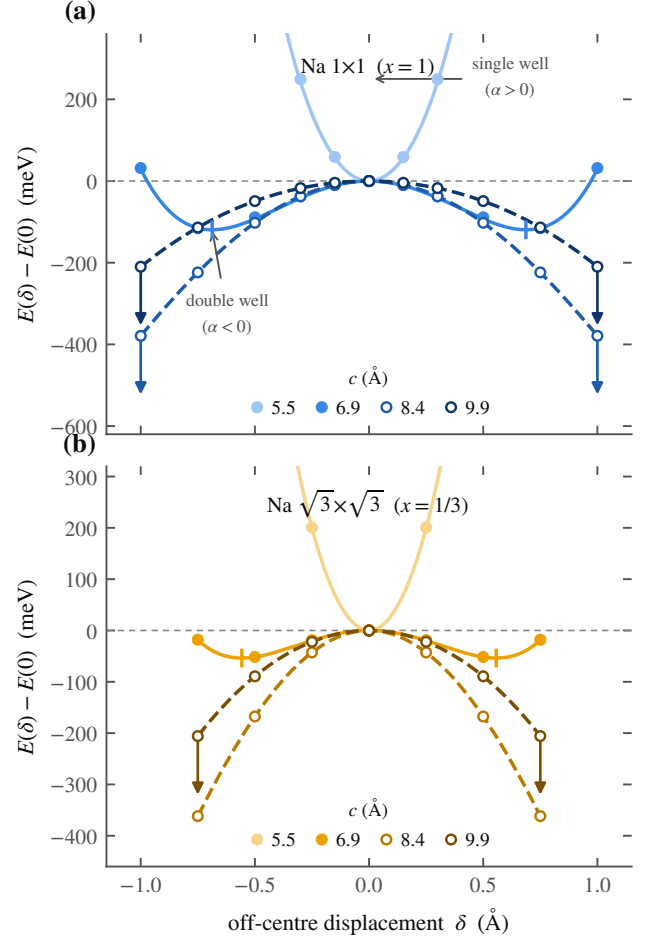
FIG. 2. The single-to-double-well transition. Energy E(\delta) of the off-centre sodium displacement, computed for \text{Na } 1 \times 1 (top, x = 1 ) and \text{Na } \sqrt{3} \times \sqrt{3} (bottom, x = 1/3 ) at the four gallery spacings; points are total energies, curves are the fits of Eq. (1) continued to sixth order where needed. At 5.5 Å the well is single and stiff ( \alpha > 0 ); by 6.9 Å it has split into a double well ( \alpha < 0 ) with minima marked. Open symbols with arrows ( c \geq 8.4 Å) flag scans that are still falling at the largest sampled displacement—there the sodium is adsorbing onto one layer and the quoted depth is only a lower bound.
