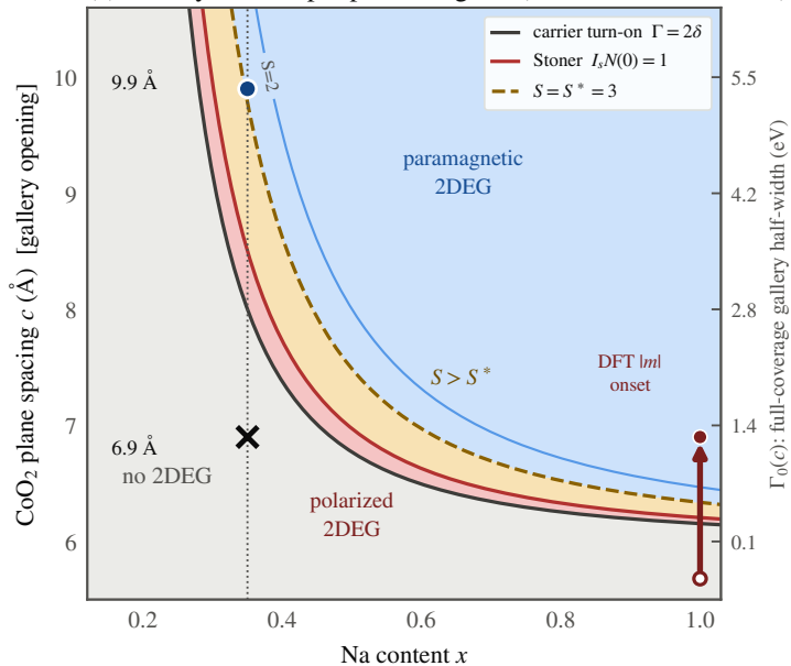
(a) Gallery-2DEG spin phase diagram (model, ansatz-labelled)
