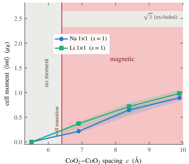
FIG. 9. The magnetic moment turning on with the well transition. Cell-integrated moment \langle |m| \rangle for Na 1 \times 1 and Li 1 \times 1 against gallery spacing; markers are the mean over the displacement scan and the bands its spread. The local moment switches on at the same spacing where \alpha turns negative, and the gallery moment is antiparallel to the cobalt. The \sqrt{3} cell is over-polarized in LSDA and is shown only as an excluded caveat band.
