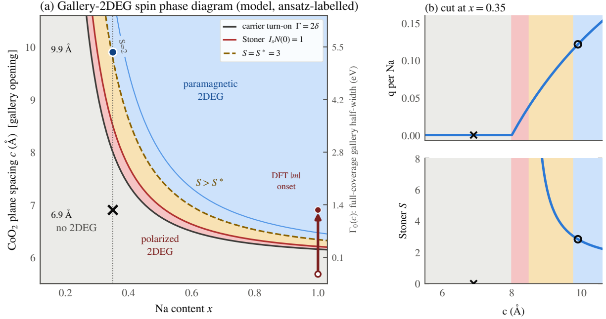
FIG. 10. The gallery-2DEG spin phase diagram. (a) Stoner phase diagram of the interlayer gas, built by carrying the SSH-type surface-charge model of Radha and Lambrecht [3] into the gallery: in the plane of Na content x and \text{CoO}_2 spacing c (right axis, the full-coverage gallery half-width \Gamma_0(c) ) the gallery band is empty below the carrier turn-on ( \Gamma = 2\delta , dark line); just above it the band is narrow and its density of states high, so the gas is Stoner-polarized (red) before widening into a paramagnon-boosted ( S > S^* , amber) and then a plain paramagnetic (blue) metal. The polarized strip hugs the turn-on line. Markers: the monolayer (6.9 Å, \times ) and bilayer (9.9 Å, \circ ) hydrates at the physical x = 0.35 ; the red bar at x = 1 marks where the DFT cell-integrated moment turns on (Fig. 9), coincident with the well transition and so with the model turn-on. The \sqrt{3} \times \sqrt{3} ( x = 1/3 ) cell is over-polarized in LSDA and excluded (the wells shift < 6\% under the spin treatment). (b) Cuts at x = 0.35 : the carrier fraction q per Na and the Stoner enhancement S against c . The model is an ansatz calibrated to the one on/off hydrate anchor pair; every parameter is source-tagged in the generating script.
