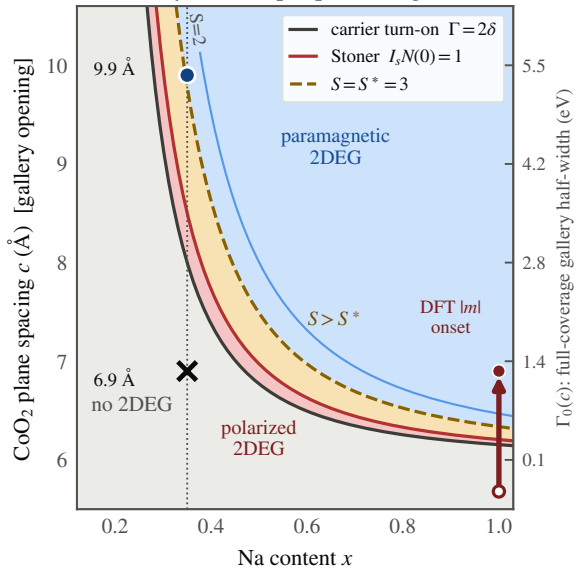
(a) Gallery-2DEG spin phase diagram
