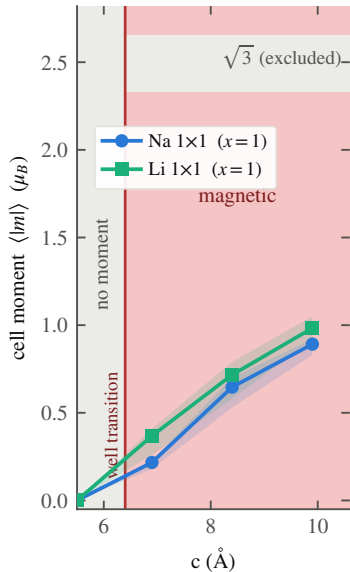
(c) DFT |m| turn-on
