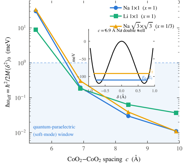
FIG. 4. The sodium mode softening. Effective zero-point frequency \hbar\omega_{\text{eff}} = \hbar^2 / 2M \langle \delta^2 \rangle_0 of the quantized alkali mode, from an exact one-dimensional solution of the fitted wells at the physical masses. It collapses by three orders of magnitude across the transition, from a stiff \sim 30 \text{ meV} single-well mode into a sub-meV soft mode as the gallery opens, entering a quantum-paraelectric window. Inset: the lowest levels in the 6.9 \text{ \AA} sodium double well, with the near-degenerate tunnelling doublet E_0, E_1 and the even overtone E_2 that carries the quadratic electron–phonon coupling.
