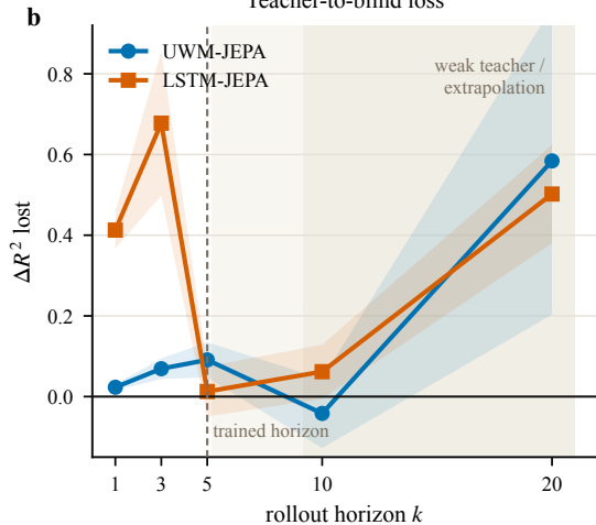
Teacher-to-blind loss
