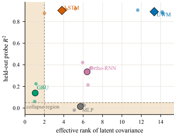
Collapse diagnostic: rank must carry task information
