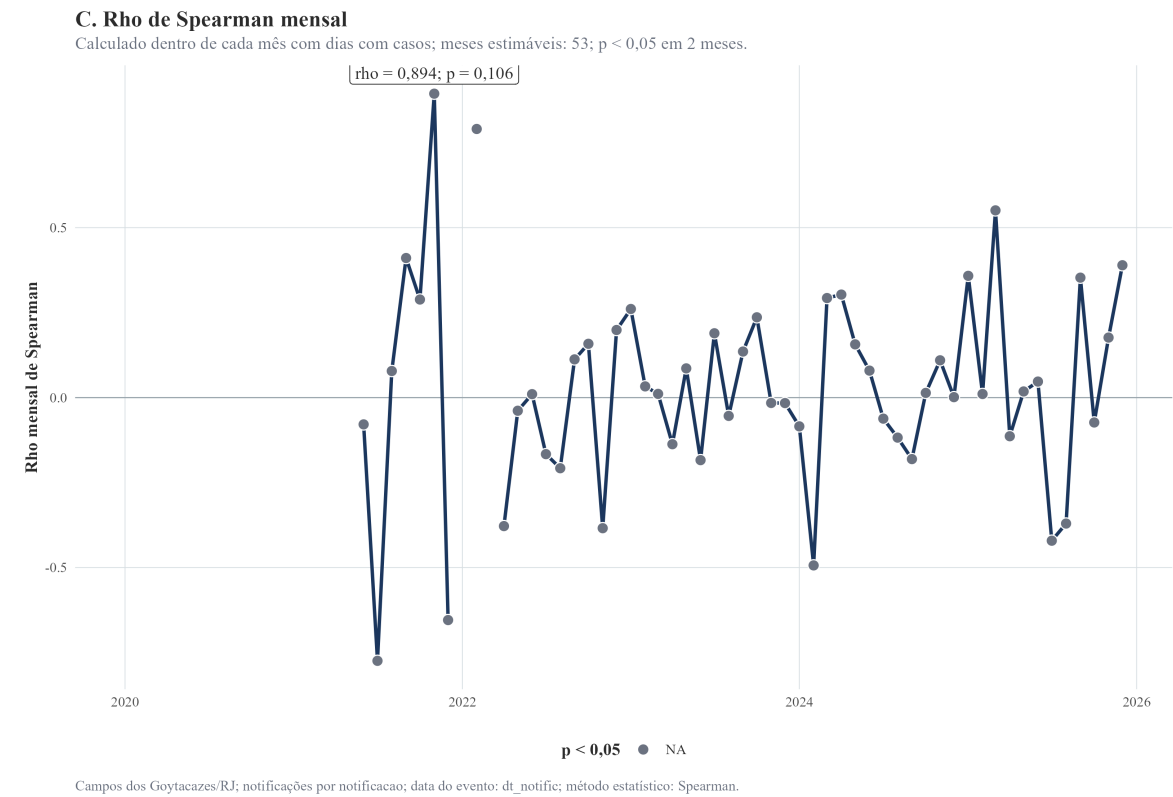
Figura 3 - Rho de Spearman mensal
