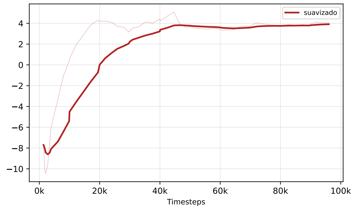
Actor Loss
