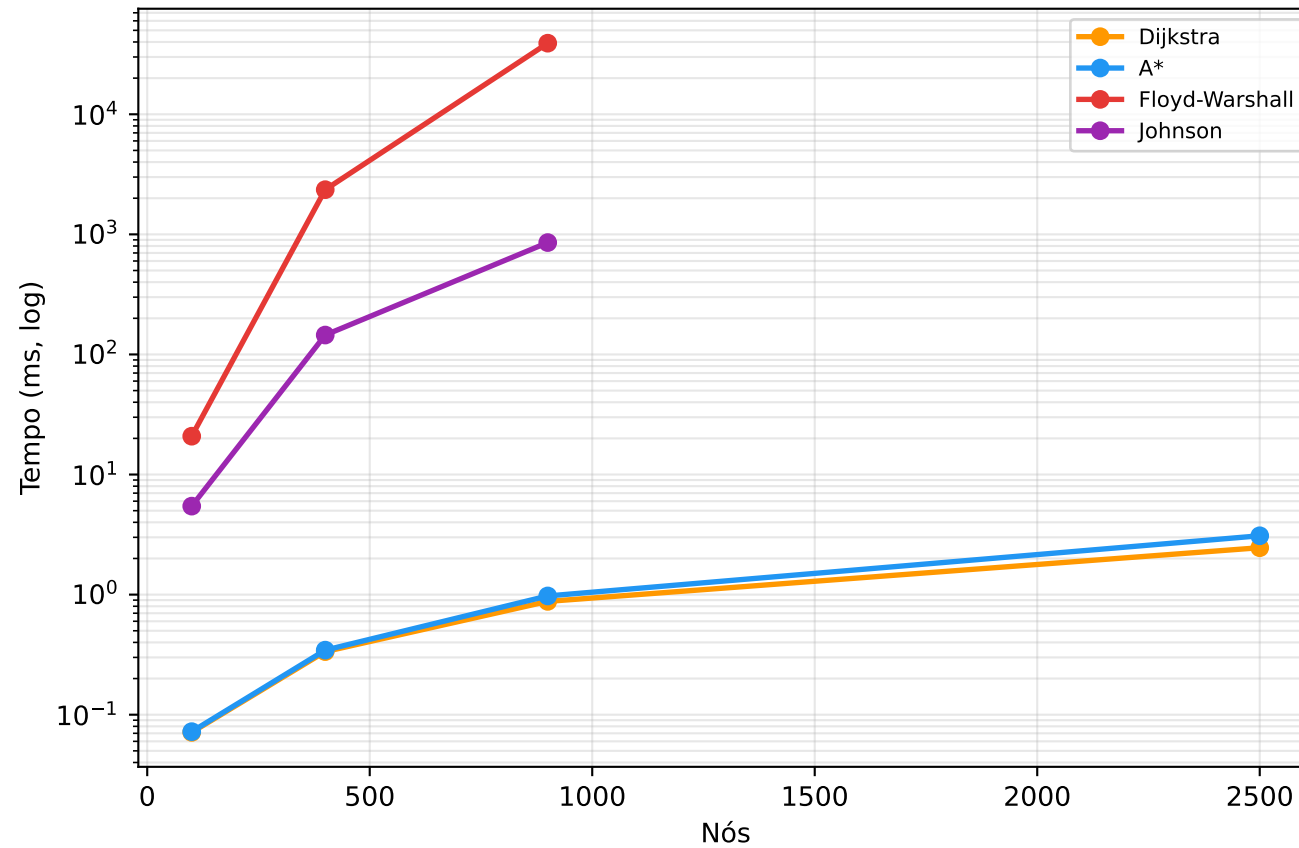
(c) Benchmark clássicos (log)
