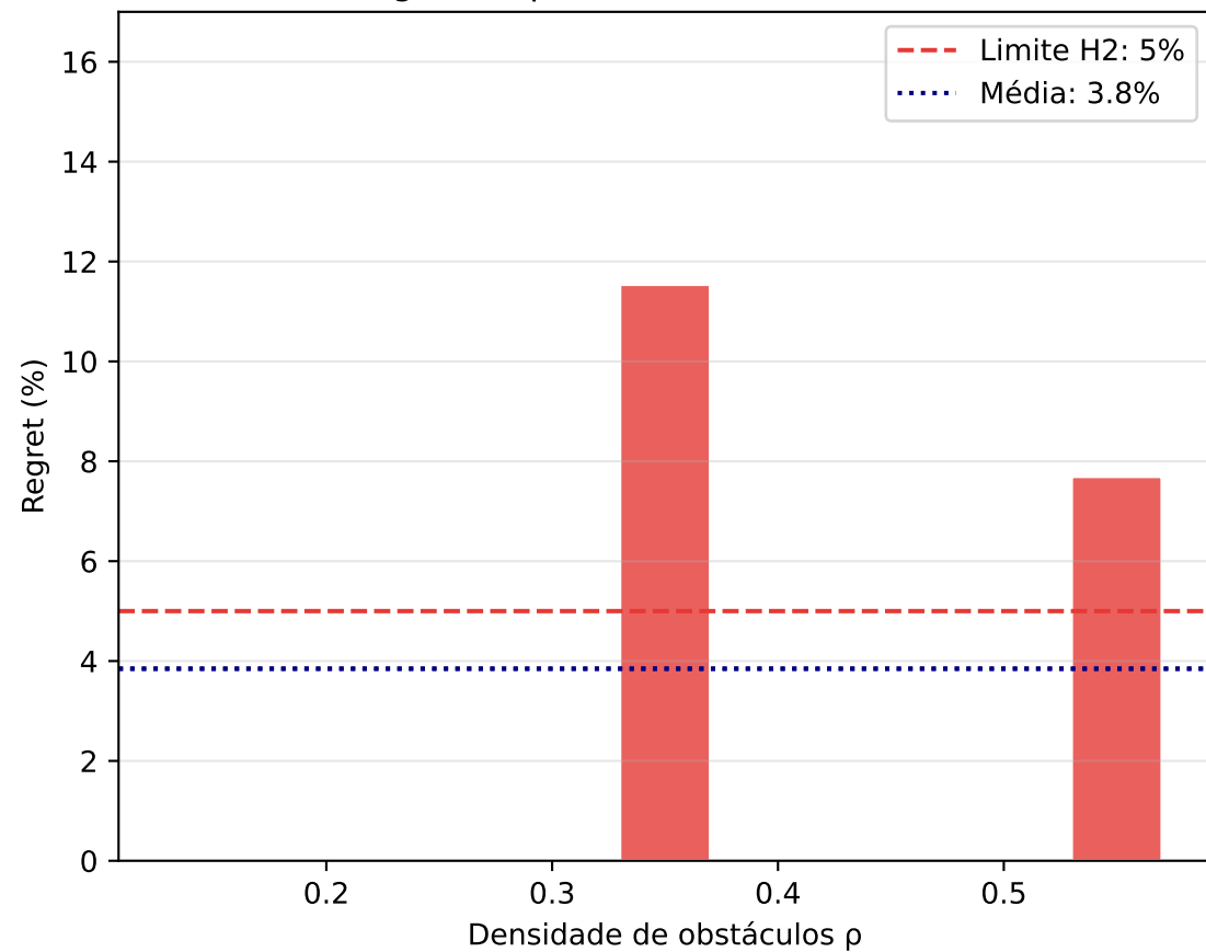
Regret do \rho -criterion vs Oracle ideal
