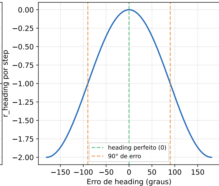
Reward de heading (contínuo) r = \cos(\text{err}) - 1 \in [-2, 0]
