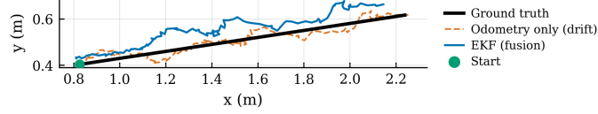
Fig. 3. Estimated trajectory under aggressive drift, Scenario 2 (straight motion). The EKF (blue) tracks ground truth (black) more closely than raw drifted odometry (orange, dashed).
