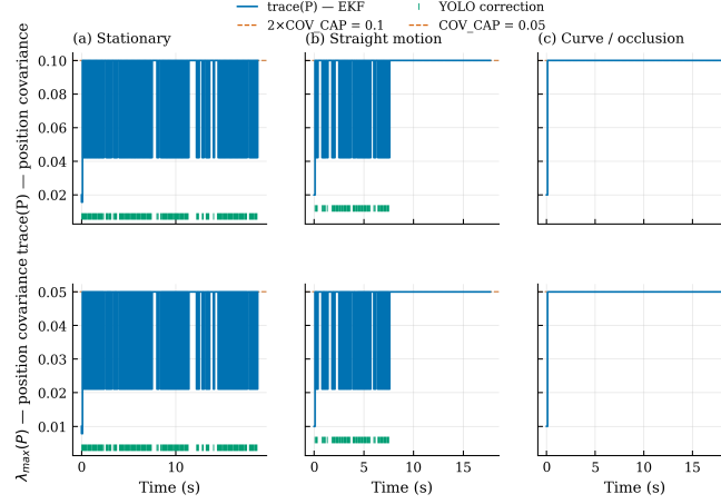
Fig. 3. \text{trace}(P_{xy}) over time (step plot), all three scenarios. Short vertical ticks along the bottom mark successful YOLO corrections. The dashed line marks 2 \times \text{COV\_CAP} = 0.1 , the ceiling on the position-covariance trace (Section 3). Coverage decreases left to right ( 27.6\% \rightarrow 11.3\% \rightarrow 0\% ), and covariance saturates at the ceiling for correspondingly longer stretches, reaching permanent saturation in the zero-coverage case.
