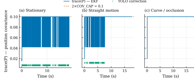
Fig. 3. \text{trace}(P_{xy}) over time (step plot), all three scenarios. Short vertical ticks along the bottom mark successful YOLO corrections. The dashed line marks 2 \times \text{COV\_CAP} = 0.1 , the ceiling on the position-covariance trace (Section 3). Coverage decreases left to right (27.6% \rightarrow 11.3% \rightarrow 0%), and covariance saturates at the ceiling for correspondingly longer stretches, reaching permanent saturation in the zero-coverage case.
