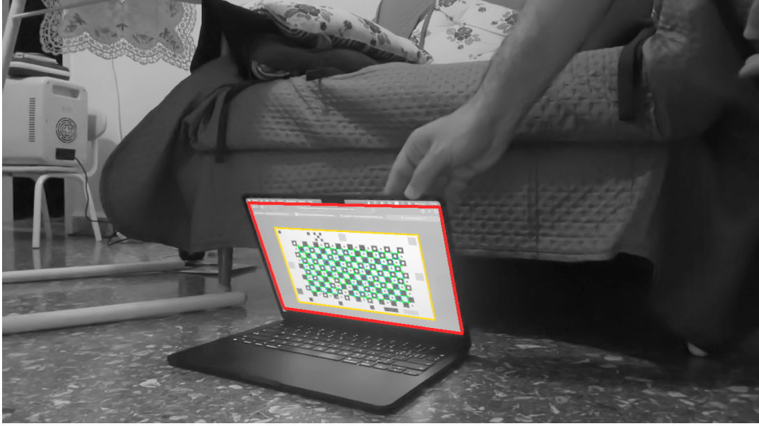
Figure 7: Everything the system detected in one real 720p webcam frame ( tools/annotate.c ). Green: 159 sub-pixel saddle corners. Cyan: the identified corner lattice. Yellow: the pattern’s 1920 \times 1080 extent mapped through the fitted homography. Red: the laptop’s lit display panel, detected by mv_display_outline ’s pattern-frame ray marching — found in the image, not assumed from a spec. The hand adjusting the lid and the couch behind do not disturb the median-based edges.
