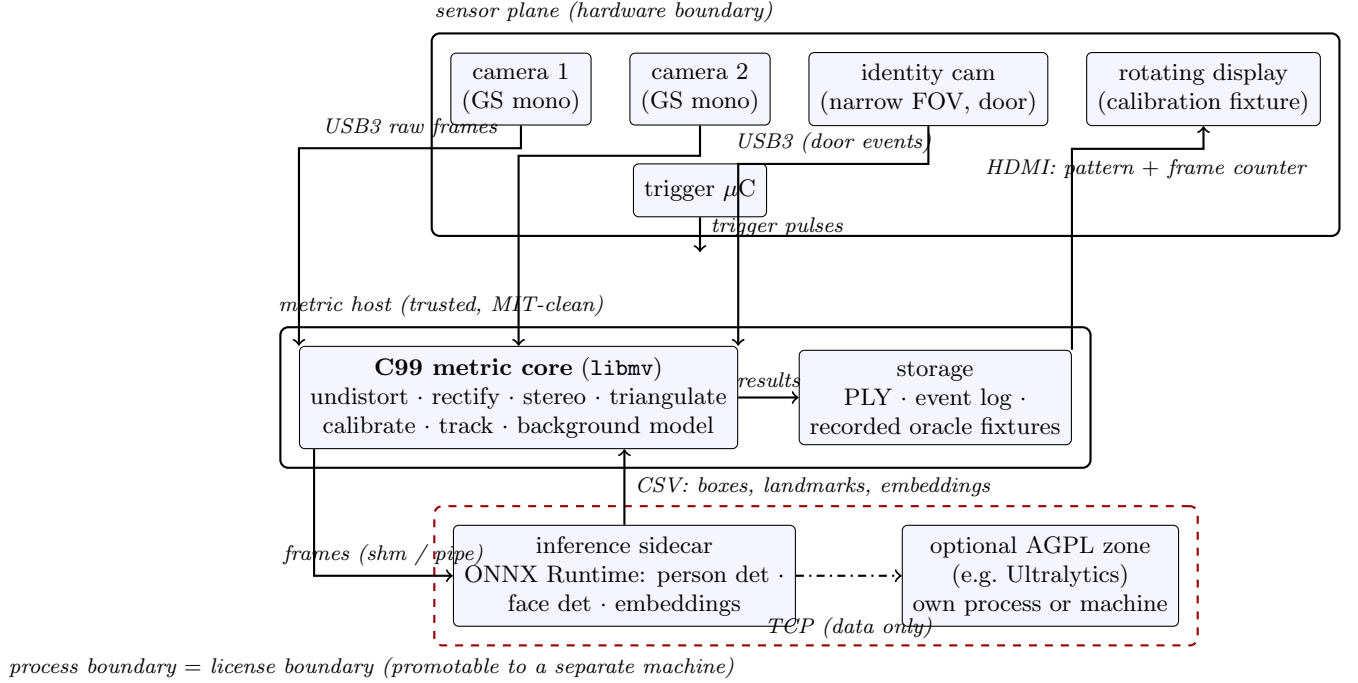
Figure 4: Deployment architecture. Solid boxes are hardware boundaries; the dashed red box is the license/process boundary — all learned components live behind it, exchanging only data (frames one way, text rows back), so it can be promoted from “separate process” to “separate machine” (a small GPU/NPU box) without any protocol change. The trigger microcontroller synchronizes both cameras, the identity camera, and — during calibration — the rotating display’s frame counter.
