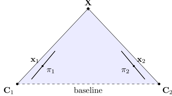
Figure 2: Epipolar geometry: the camera centers C_1, C_2 and the scene point X span the epipolar plane (shaded); its intersections with the image planes \pi_1, \pi_2 are the corresponding epipolar lines on which x_1 and x_2 must lie.
