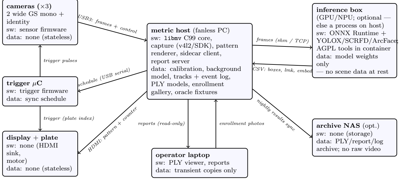
Figure 3: Machine-centric deployment view: per-machine software and persistent data, and all inter-machine flows. Scene and identity data rest only on the metric host; the inference box is compute-only; sensors and fixtures are stateless.
