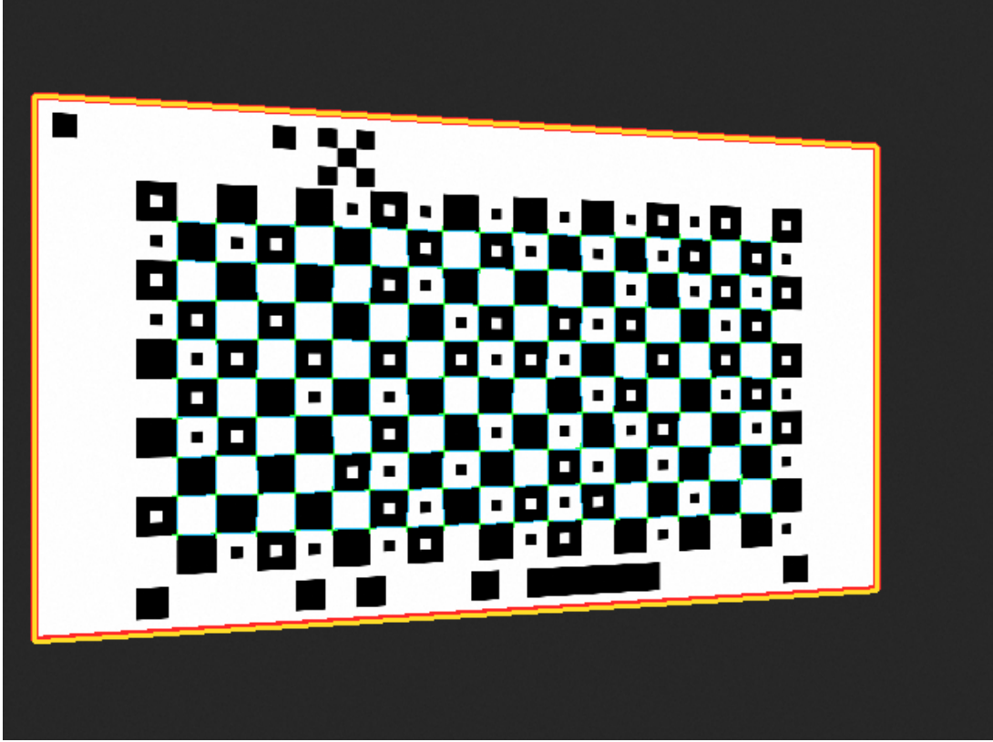
Figure 13: Everything the system detects in one frame ( tools/annotate.c ), shown on a synthetic pattern view ( tools/genframes.c ; 162 corners, counter decoded): the original 720p webcam frame — 159 sub-pixel saddle corners, with a hand adjusting the lid and a couch behind that did not disturb the median-based edges — is imagery of the author’s home and is withheld from the public repository. Overlays are identical in kind: green sub-pixel saddle corners, cyan identified lattice, yellow pattern extent mapped through the fitted homography, red the lit display panel detected by mv_display_outline ’s pattern-frame ray marching — found in the image, not assumed from a spec.
