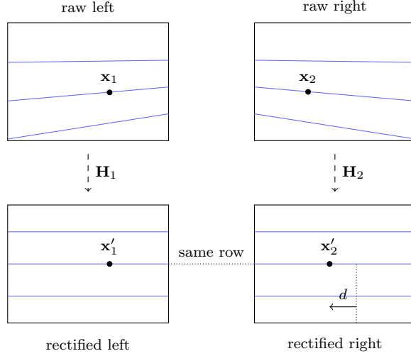
Figure 5: Rectification. Top: in the raw pair the epipolar lines (blue) of Figure 4 are slanted and unaligned, so the match of a pixel \mathbf{x}_1 must be sought along a slanted line. Bottom: the precomputed homographies \mathbf{H}_1, \mathbf{H}_2 warp each image so that epipolar lines become horizontal and row-aligned between the views; the same scene point now lands on the same row in both images (dotted), displaced only horizontally by the disparity d (dotted vertical: the column \mathbf{x}'_1 would occupy at infinite depth).
