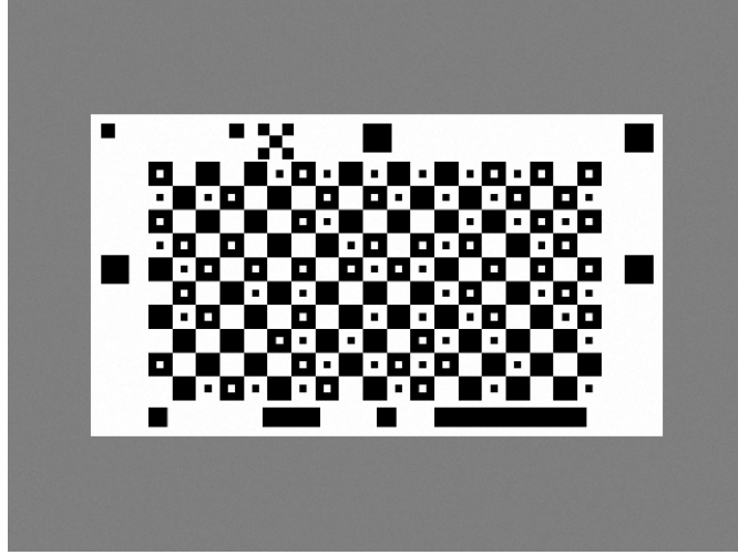
Figure 9: What the reader sees: rendered frontal view of the spec-v1 screen (pose 0 of Table 7) — saddle grid with M-array dots, counter strip (bottom), version block and fine grid (top), phase patches; from demo_patternsim ’s PGM output.
