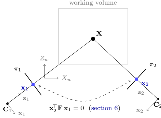
Figure 2: The camera model, drawn for the rig. The volume and the scene point \mathbf{X} live in the world frame (gray axes X_w, Z_w ; Y_w out of the page). Each camera i carries its own frame — optical axis \mathbf{z}_i , image axis \mathbf{x}_i, \mathbf{y}_i out of the page — related to the world by (\mathbf{R}_i, \mathbf{t}_i) , and its intrinsic matrix \mathbf{K}_i turns the intersection of a viewing ray (solid arrow) with the image plane \pi_i (thick) into a pixel \mathbf{x}_i (blue). Because both cameras watch the same volume, the two pixels of one scene point are not independent: knowing \mathbf{x}_1 confines \mathbf{x}_2 to the image of \mathbf{x}_1 ’s back-projected ray (dashed relation), which section 6 makes exact as the fundamental-matrix constraint.
