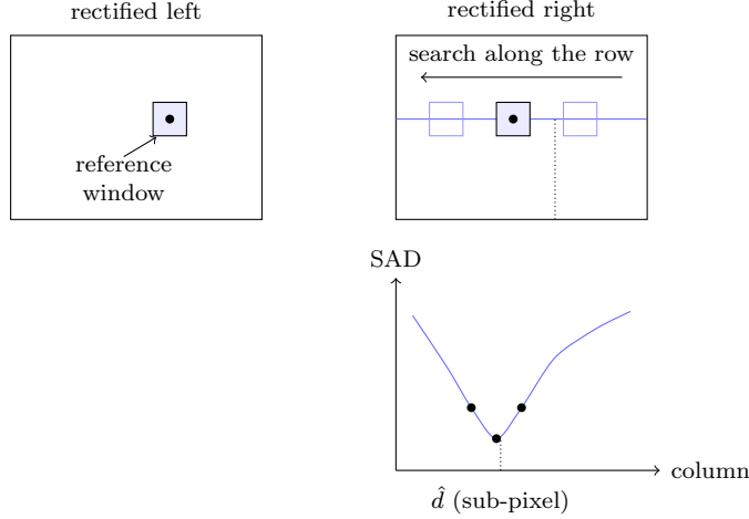
Figure 6: Block matching on the rectified pair. Top: the (2w+1)^2 -pixel window around a left pixel is compared against same-size windows sliding along the single corresponding right row (blue); light squares are candidates, the shaded one is the best match, and the dotted vertical repeats the reference column so the displacement is visible. Bottom: SAD cost of each candidate column; the three dots are the integer samples around the minimum, and a parabola through them places the sub-pixel disparity \hat{d} .
