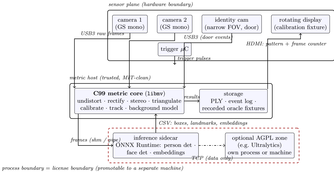
Figure 14: Deployment architecture. Solid boxes are hardware boundaries; the dashed red box is the license/process boundary — all learned components live behind it, exchanging only data (frames one way, text rows back), so it can be promoted from “separate process” to “separate machine” (a small GPU/NPU box) without any protocol change. The trigger microcontroller synchronizes both cameras, the identity camera, and — during calibration — the rotating display’s frame counter.
