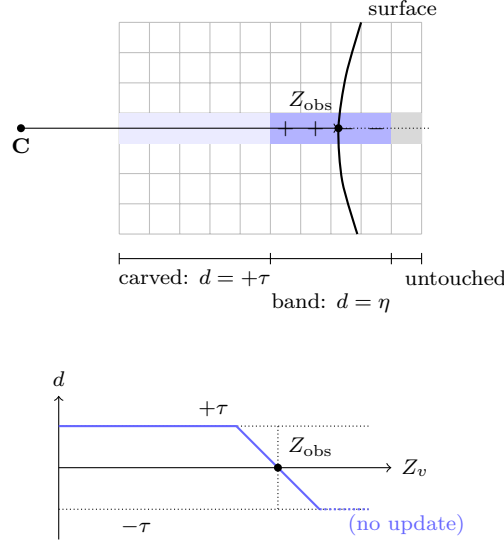
Figure 7: One depth measurement seen by the TSDF, in the grid (top) and as a function (bottom). Top: a slice of the voxel grid; along the ray from the camera center \mathbf{C} to the observed surface hit Z_{\text{obs}} , voxels well in front of the surface are carved with the clamped value +\tau (light blue), voxels inside the truncation band store the true signed offset \eta (darker blue, sign marked), and voxels more than \tau behind the surface are left untouched (gray) — the surface (thick curve) is later recovered as the zero crossing between the + and - cells. Bottom: the same rule (17) as the truncated signed distance d stored at a voxel of depth Z_v along the ray; the blue profile is what one measurement contributes, and fusion averages many such profiles per voxel.
