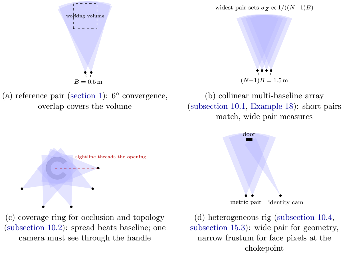
Figure 8: Camera-positioning scenarios, top-down, frustums drawn as viewing wedges (range truncated for the page; the real frusta extend with distance). Overlap density shows where triangulation is possible.
