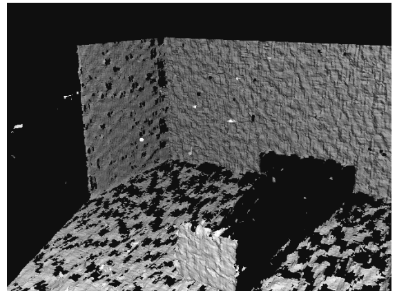
(f) the reconstruction , same viewpoint as (e): floor, both walls, the box, and its occlusion shadow behind it; holes are honestly-unobserved regions (texture-gated grazing floor, occlusions); granularity is the 15 mm voxel grid
