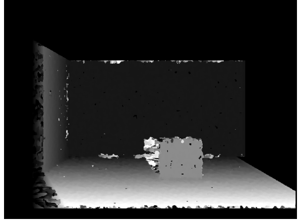
(b) disparity: bright = near (floor sweeping toward the camera), dark = far (back wall); black = gated invalid — the texture desert above the walls and occlusion fringes beside the box, exactly the failure modes section 8 predicts
