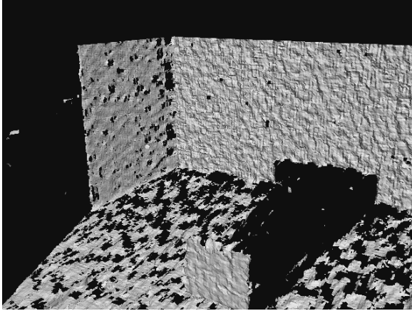
(c) the reconstructed mesh, shaded and rendered from a viewpoint no camera occupies: floor, both walls, the box, and its occlusion shadow behind it; holes are honestly-unobserved regions (texture-gated grazing floor, occlusions), granularity is the 15 mm voxel grid
