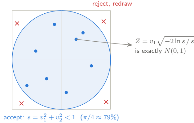
Figure 6: The polar Box–Muller sampler: uniform points in the square are kept only if they land in the disc; the kept point’s radius and direction are then reshaped into a standard normal. Rejection turns an easy distribution (uniform on a square) into a hard one (uniform on a disc) at a known, modest cost. [ interactive version on the web ]
