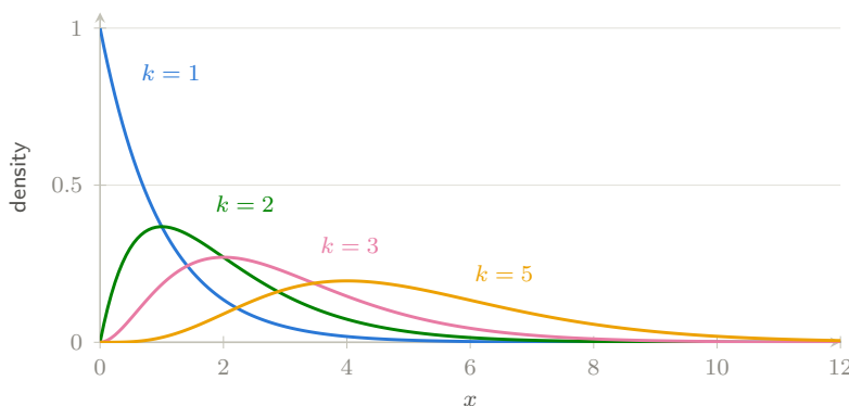
Figure 7: Gamma densities with scale \theta = 1 . Shape k = 1 is the exponential; as k grows the density moves right, symmetrizes, and (by the CLT, since it is a sum of k waits) approaches a normal — the family tree of Figure 1 in a single picture. [ interactive version on the web ]
