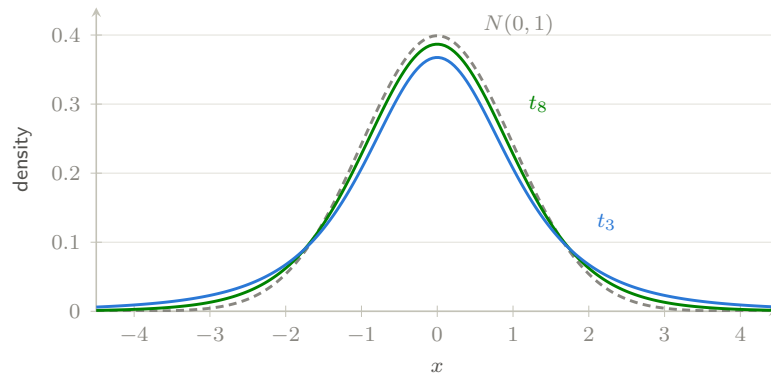
Figure 9: Student’s t against the standard normal. The lower the degrees of freedom, the more probability escapes into the tails — so small samples need larger observed effects before a result counts as surprising. This gap between t_\nu and N(0,1) is the small-sample correction of §5. [interactive version on the web]
