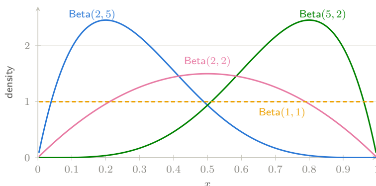
Figure 8: Beta densities: the driver’s worked example \text{Beta}(2, 5) leans toward small proportions, its mirror \text{Beta}(5, 2) toward large ones, \text{Beta}(2, 2) is a symmetric hump, and \text{Beta}(1, 1) is the uniform — the natural “know nothing” prior for a probability. [interactive version on the web]
