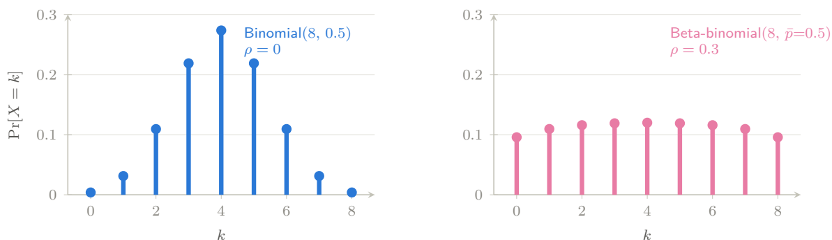
Figure 5: The same eight flips at the same mean rate, differing only in where the coin comes from. Left: one coin for everyone — the binomial concentrates on four heads. Right: a coin drawn per unit with intraclass correlation \rho = 0.3 — the mean is unmovable at 4, but the mass has fled to the extremes, because a unit that drew a high p tends to produce a run. The variance ratio is 1 + (n - 1)\rho = 3.1 . [interactive version on the web]
