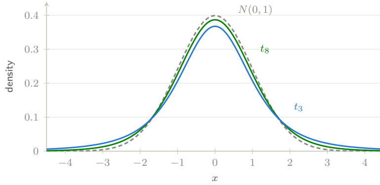
Figure 11: Student’s t against the standard normal. The lower the degrees of freedom, the more probability escapes into the tails — so small samples need larger observed effects before a result counts as surprising. This gap between t_\nu and N(0,1) is the small-sample correction of §5. [ interactive version on the web ]
