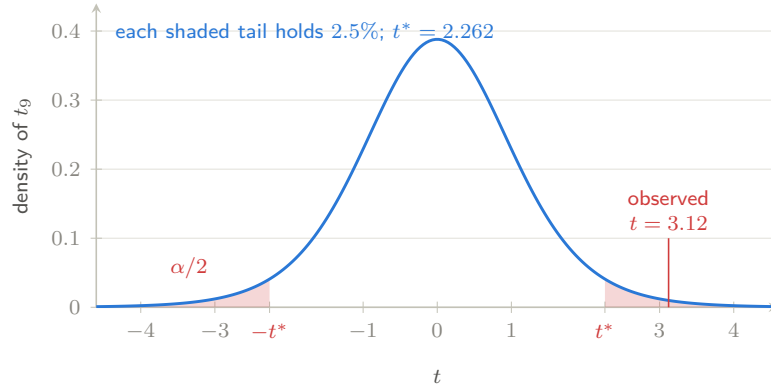
Figure 12: The one-sample t -test on the repository’s own test fixture ( n = 10 , df = 9 ). Under H_0 the statistic follows the blue t_9 density; the shaded tails beyond \pm t^* are the 5% rejection region, and the observed t = 3.12 lands past them, giving the two-sided p -value 0.012 — the total tail area beyond \pm 3.12 . [interactive version on the web]
