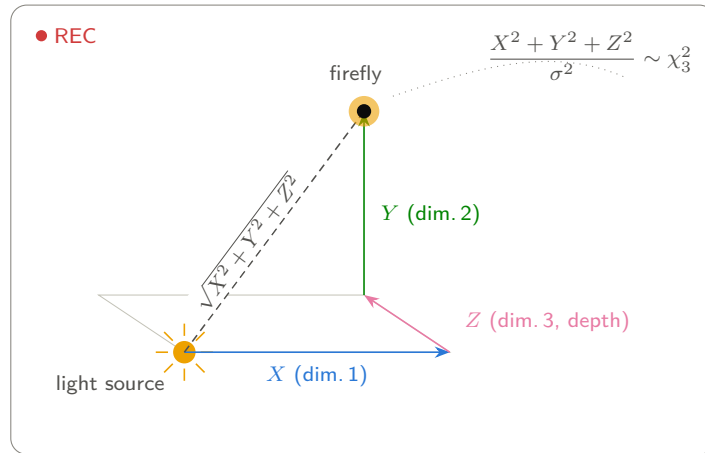
Figure 10: One frame of the firefly video: the k = 3 picture of \chi^2 . The firefly's deviations from the light source — horizontal X , vertical Y , and depth Z — are the three independent N(0, \sigma^2) dimensions of k = 3 ; their squared, \sigma -scaled sum is \chi_3^2 (mean 3, variance 6), and the dashed distance to the bulb is the scaled \chi_3 of Maxwell's speed law. The dotted trail is the flight path across earlier frames.
