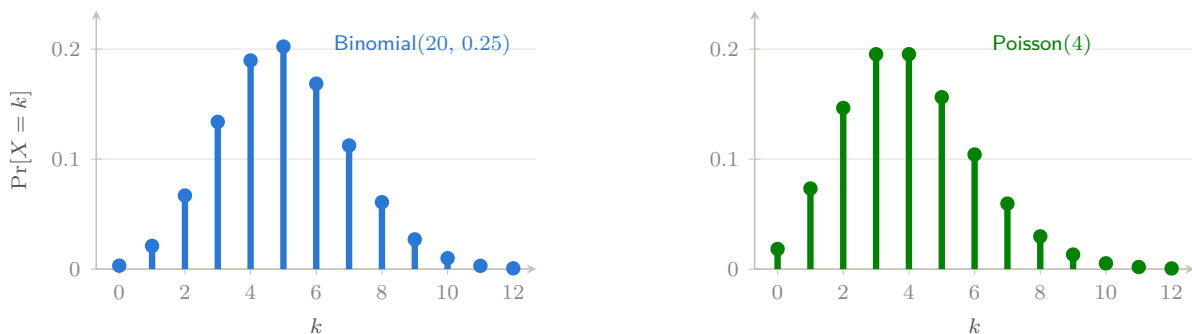
Figure 4: The two classical count laws, at the driver’s worked parameters. Both have mean \approx 4 –5, but the binomial is confined to \{0, \dots, 20\} while the Poisson has an unbounded right tail — the visible signature of “many opportunities, each rare”. [interactive version on the web]
