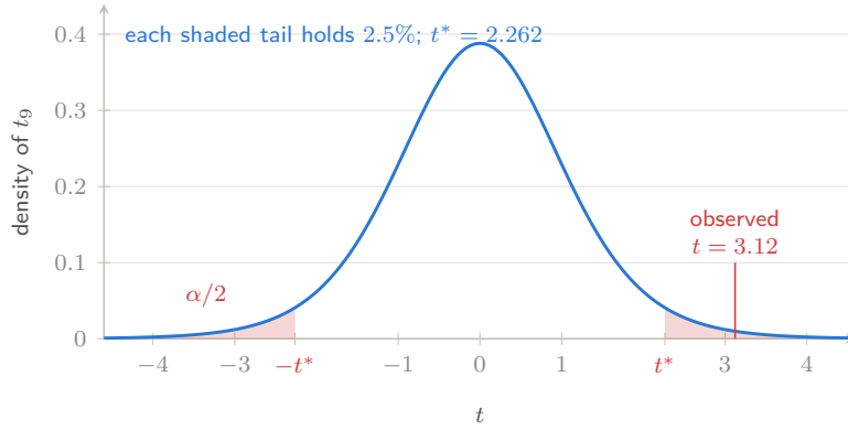
Figure 13: The one-sample t -test on the repository’s own test fixture ( n = 10 , df = 9 ). Under H_0 the statistic follows the blue t_9 density; the shaded tails beyond \pm t^* are the 5% rejection region, and the observed t = 3.12 lands past them, giving the two-sided p -value 0.012 — the total tail area beyond \pm 3.12 . [interactive version on the web]
