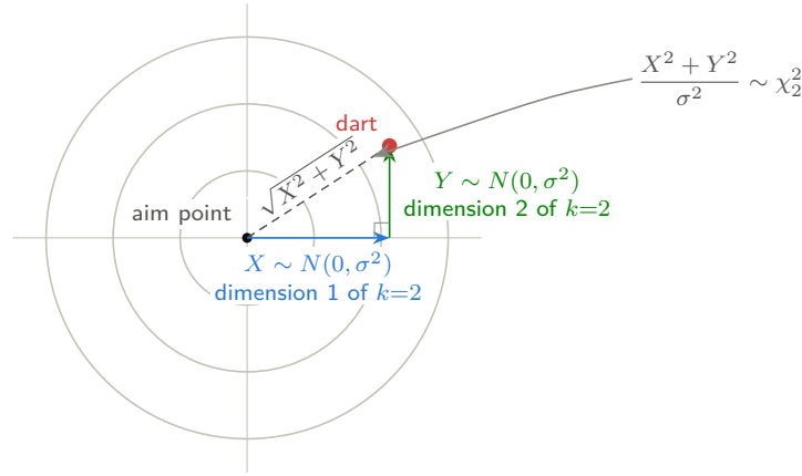
Figure 10: The dartboard geometry of \chi_2^2 . The dart's horizontal and vertical deviations from the aim point, X and Y , are independent N(0, \sigma^2) errors — they are the k = 2 dimensions being summed. Their squared, \sigma -scaled sum is \chi_2^2 (mean 2, variance 4), while the miss radius \sqrt{X^2 + Y^2} is the Rayleigh of §4.9. A clamped rifle's proof target is read with exactly this geometry, once per round fired.
