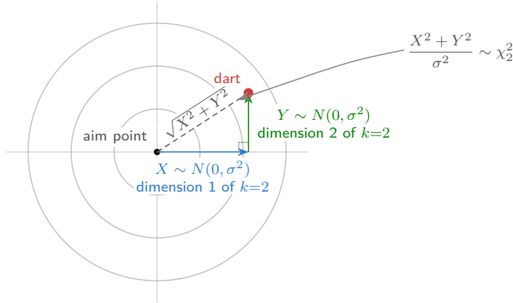
Figure 9: The dartboard geometry of \chi_2^2 . The dart's horizontal and vertical deviations from the aim point, X and Y , are independent N(0, \sigma^2) errors — they are the k = 2 dimensions being summed. Their squared, \sigma -scaled sum is \chi_2^2 (mean 2, variance 4), while the miss radius \sqrt{X^2 + Y^2} is the Rayleigh of §4.9. A clamped rifle's proof target is read with exactly this geometry, once per round fired.
