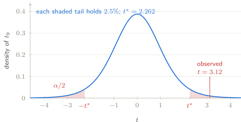
Figure 12: The one-sample t -test on the repository’s own test fixture ( n = 10 , \text{df} = 9 ). Under H_0 the statistic follows the blue t_9 density; the shaded tails beyond \pm t^* are the 5% rejection region, and the observed t = 3.12 lands past them, giving the two-sided p -value 0.012 — the total tail area beyond \pm 3.12 . [ interactive version on the web ]
