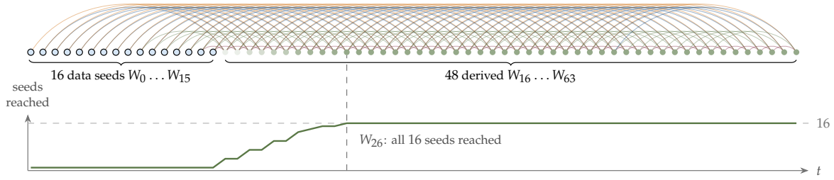
Figure 6: The message schedule as a computed dependency graph (generated by tools/wschedule_graph.py , which also emits a Graphviz .dot version). Nodes are the 64 schedule words in index order; the sixteen data-carrying seeds W_0, \dots, W_{15} are blue, and derived words darkened with the number of seeds they transitively depend on. Each of the four arc colours is one term of W_t = \sigma_1(W_{t-2}) \boxplus W_{t-7} \boxplus \sigma_0(W_{t-15}) \boxplus W_{t-16} . The lower trace counts seeds reached versus t ; it reaches all sixteen at W_{26} (dashed line), after which the message is fully diffused through the schedule alone.
