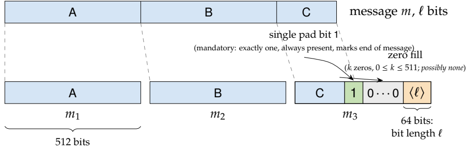
Figure 2: Padding and blocking, for a message needing k = 3 blocks. The linear message (blue; portions A, B, C) is consumed left to right by 512-bit blocks. The final block is completed by a single 1 bit (green), a run of 0s, and the 64-bit binary encoding of the message length \ell (orange)—the Merkle–Damgård strengthening. The rule is exact and admits no options: to a message of \ell bits one always appends one 1, then the fewest 0s (possibly none) so that the total reaches a multiple of 512 once the 64-bit length is affixed—i.e. k is the least \geq 0 solution of \ell + 1 + k + 64 \equiv 0 \pmod{512} . The 1 bit and the length field are never omitted; only the zero-count k depends on \ell , and if the tail C leaves no room for the 65 closing bits, k simply runs on into an extra all-padding block.
