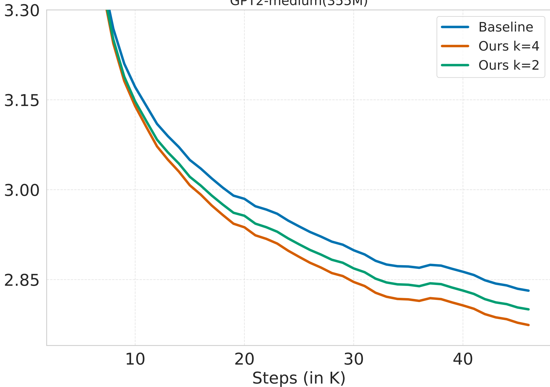
GPT2-medium(355M)
