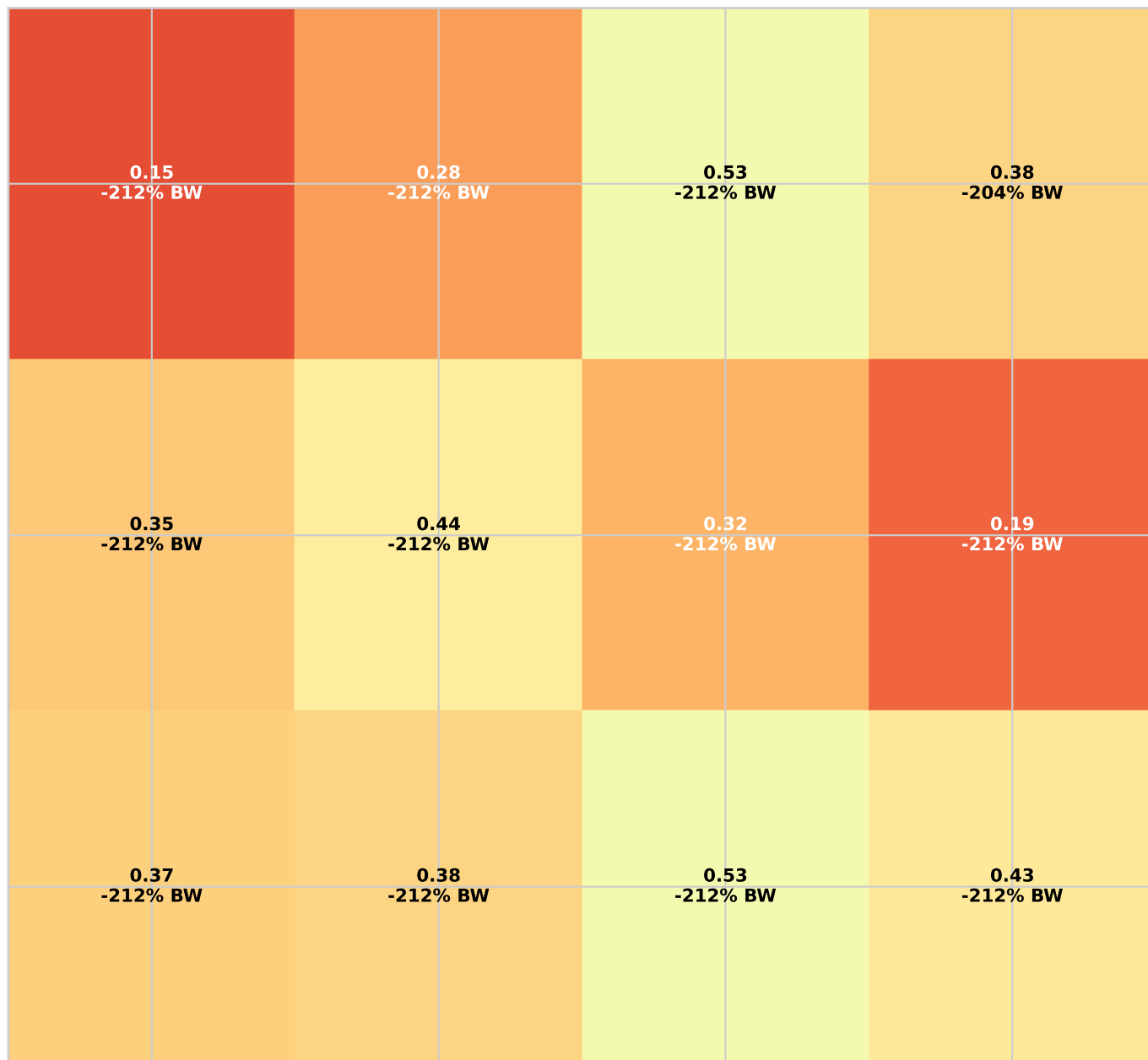
Semantic fidelity heatmap (clinical state F1 by network × command)
