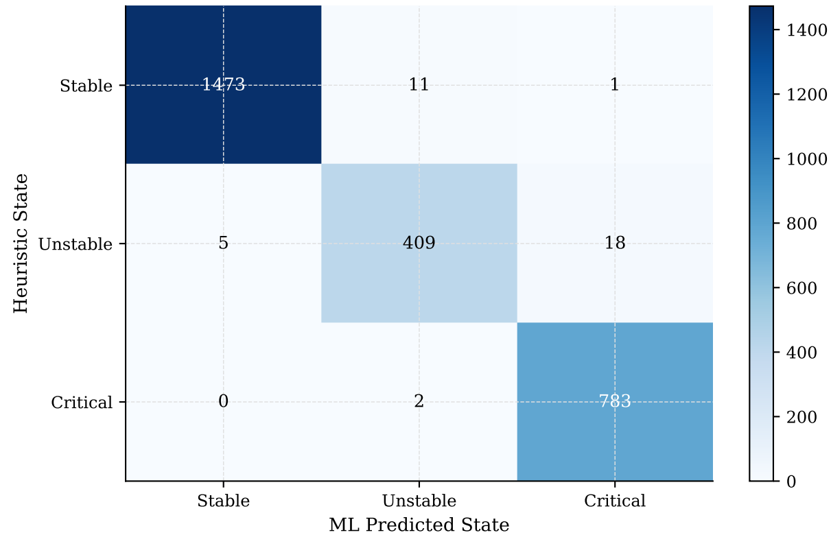
Confusion Matrix (agreement=98.6%)
