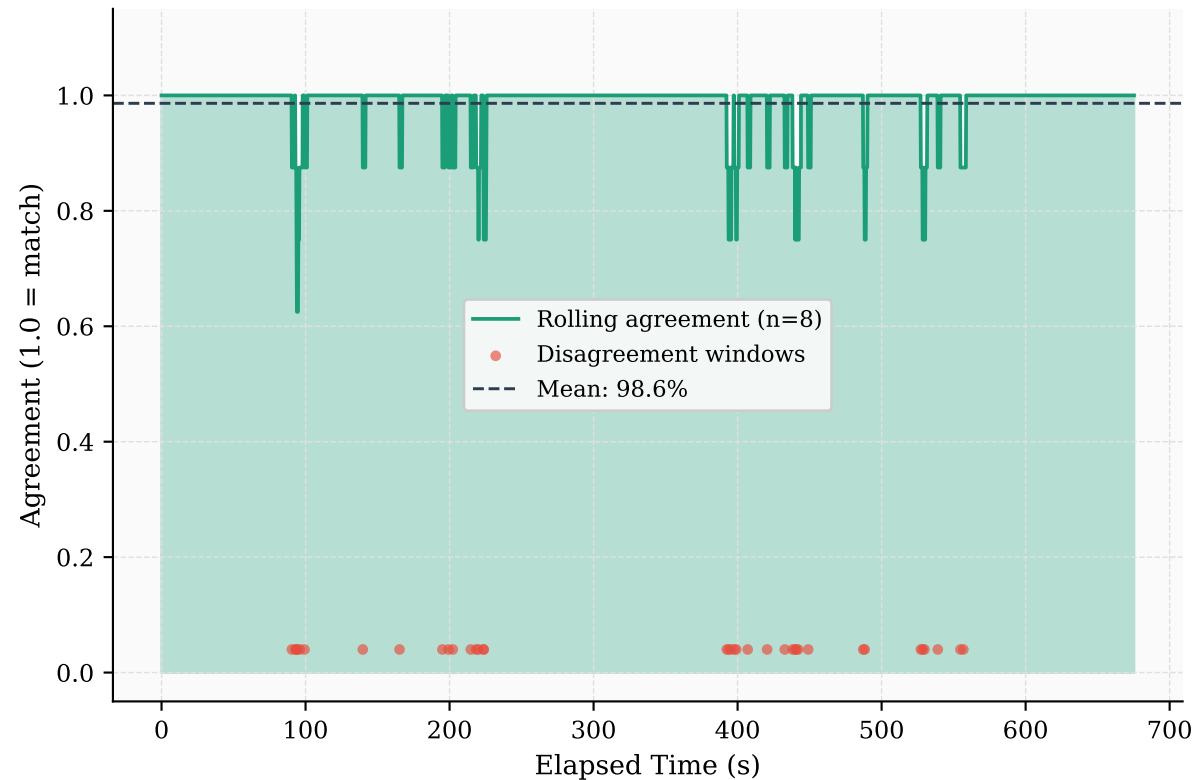
ML vs Heuristic Agreement over Time (Overall: 98.6%)
