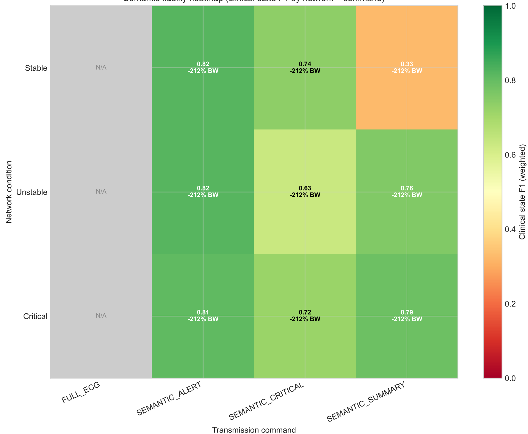
Semantic fidelity heatmap (clinical state F1 by network × command)
