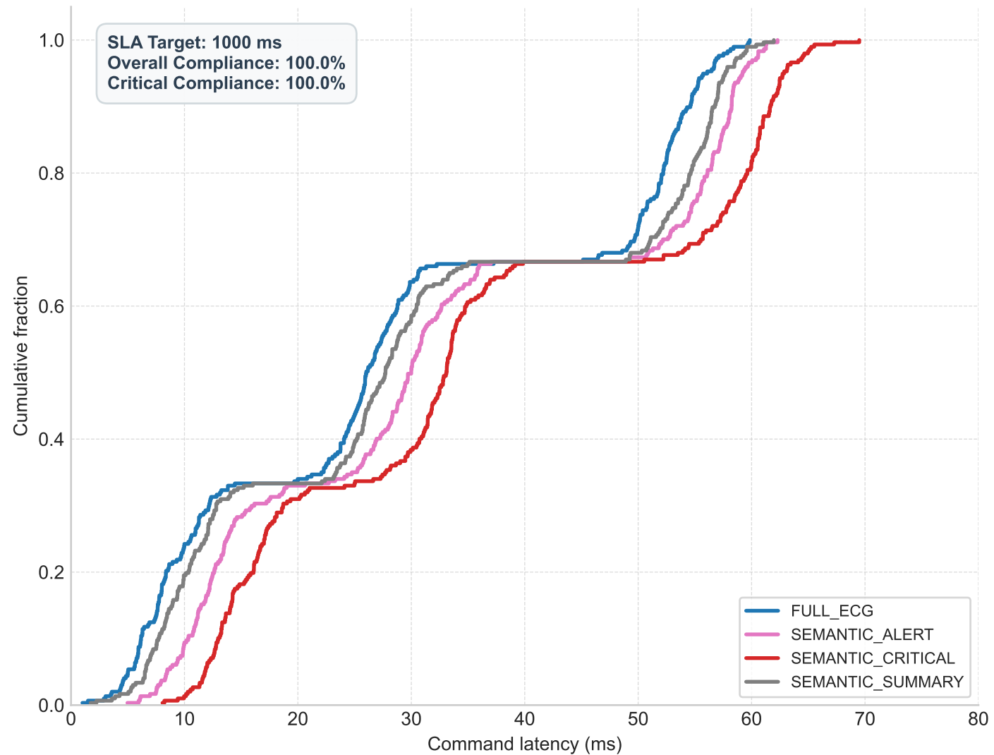
Command Latency CDF by Command Type
