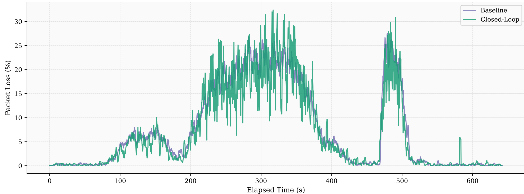
Packet Loss: Baseline vs Closed-Loop (same netem stress scenario, different response)
