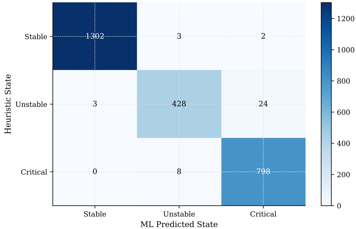
Confusion Matrix (agreement=98.4%)
