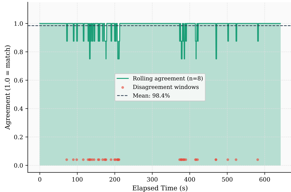
ML vs Heuristic Agreement over Time (Overall: 98.4%)
