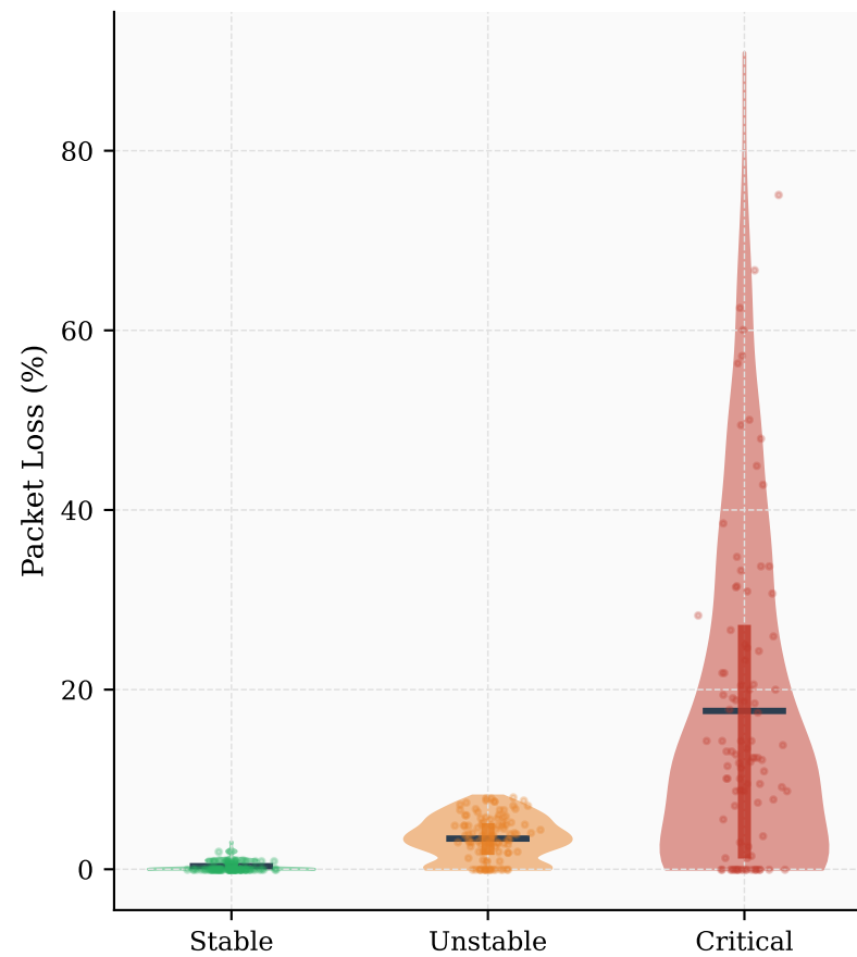
Packet Loss
