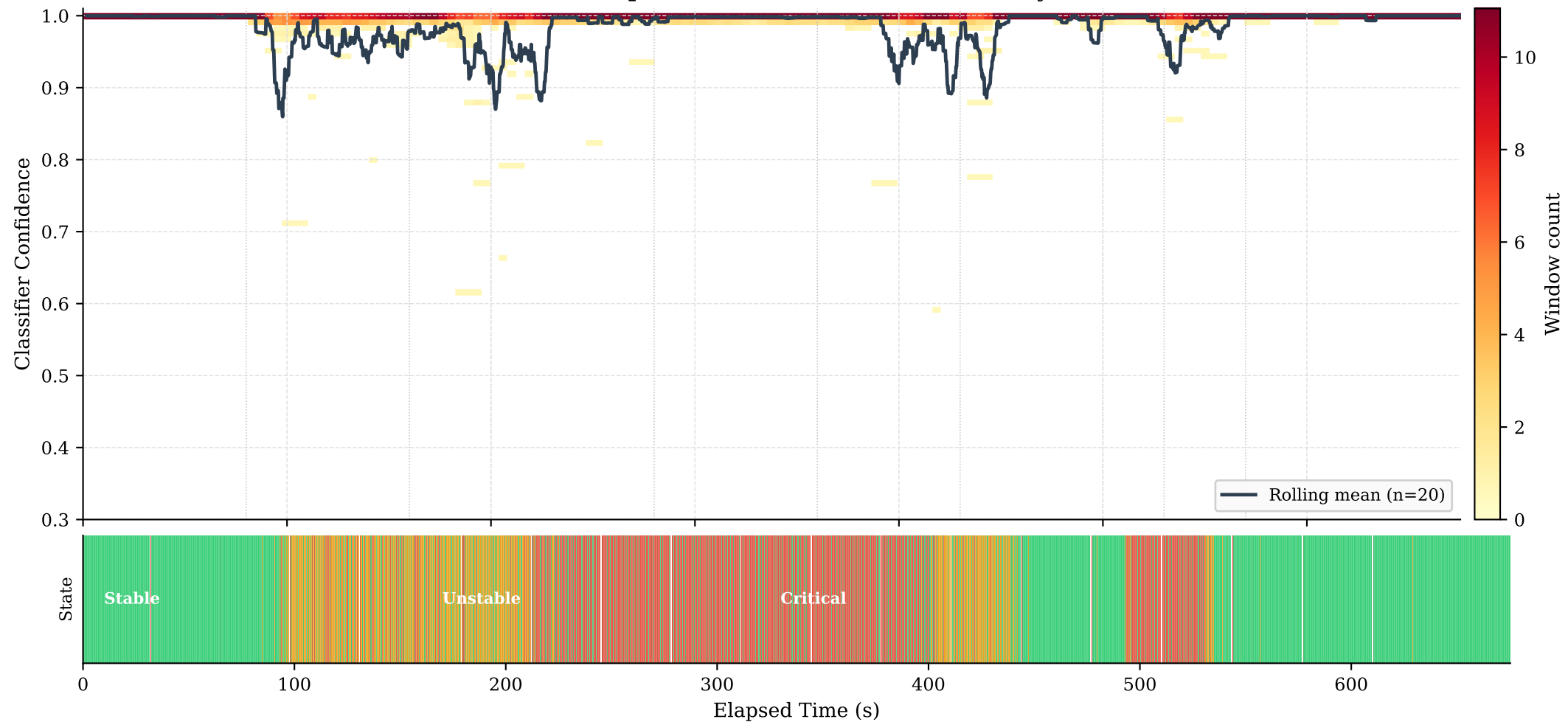
Closed-Loop — Prediction Confidence Density
